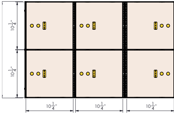
SS-6PV3 6 - 10 x 10 Stainless Steel Doors
