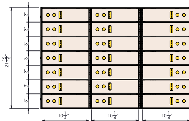
SS-3PV3 21 - 3 x 10 Stainless Steel Doors
