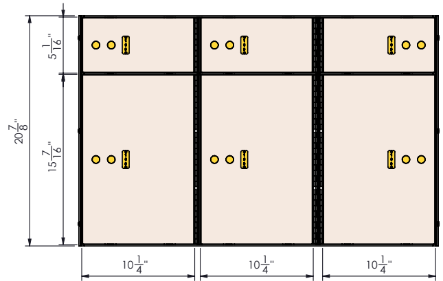
SS-7PV3 3 - 5 x 10 Stainless Steel Doors 3 - 15 x 10 Stainless
