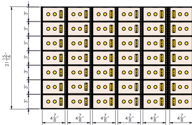
SS-1PV3 42 - 3 x 5 Stainless Steel Doors
