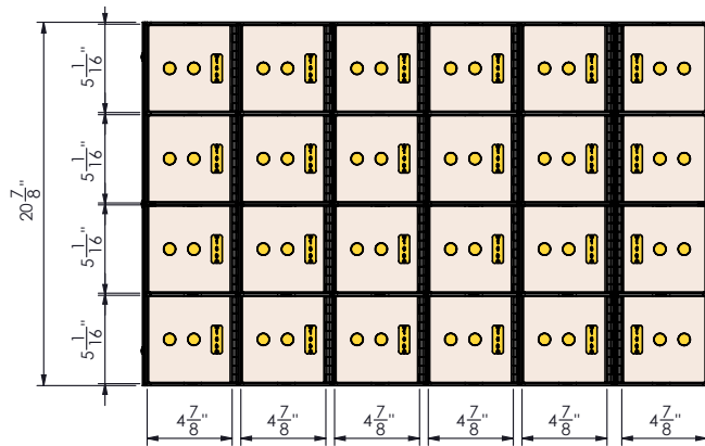
SS-2PV3 24 - 5 x 5 Stainless Steel Doors
